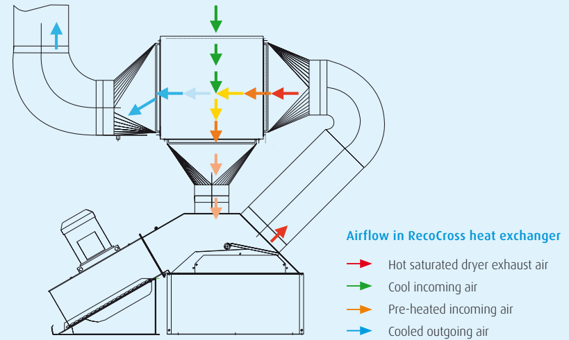
Senking dryers with RecoCross heat exchangers
