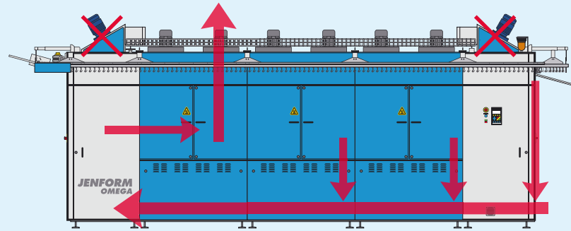
Energy-optimising air recirculation in the new Omega Pro Gas.
